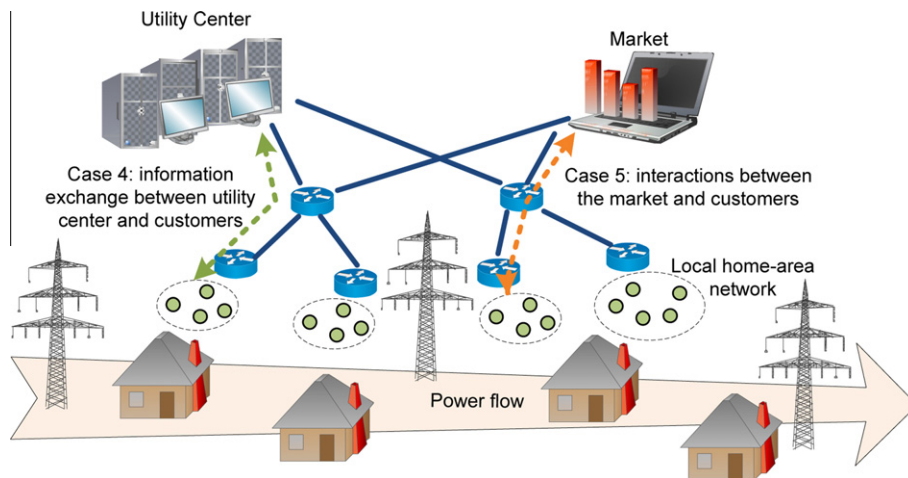
Fig. 4. Key use cases in the AMI and home-area networks.
