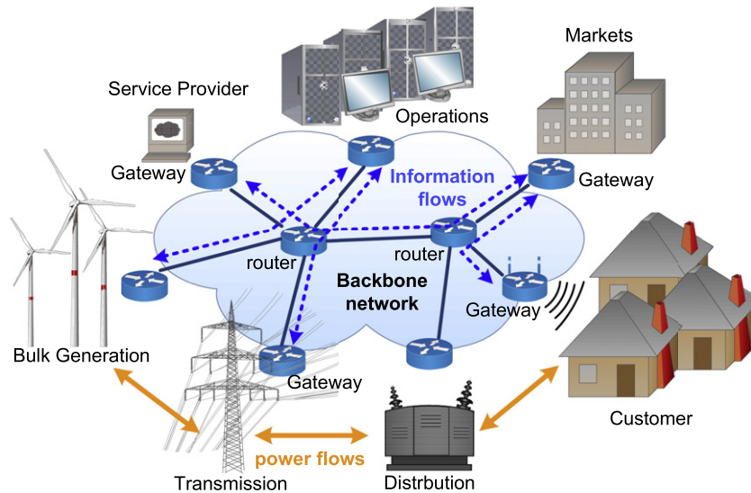
Fig. 1. The network architecture in the Smart Grid: backbone and local-area networks.
