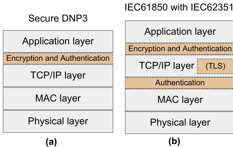
Fig. 9. Secure DNP3 and IEC 61850 with IEC 62351.
