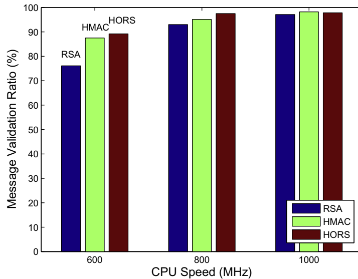
(a) Communication performance of authentication protocols for GOOSE messaging as a function of CPU speed. The packet size is fixed to 400 bytes.
